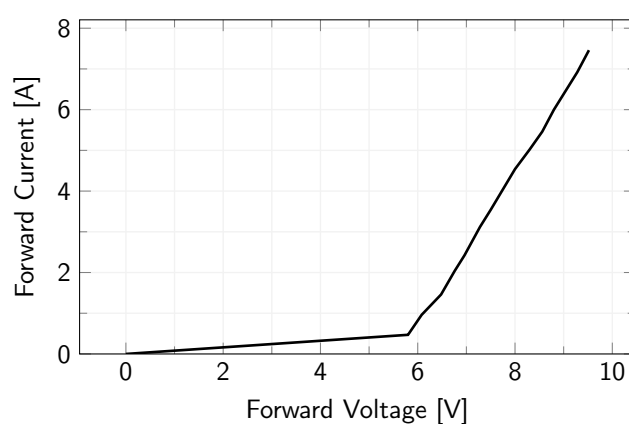
Forward Current Characteristics
